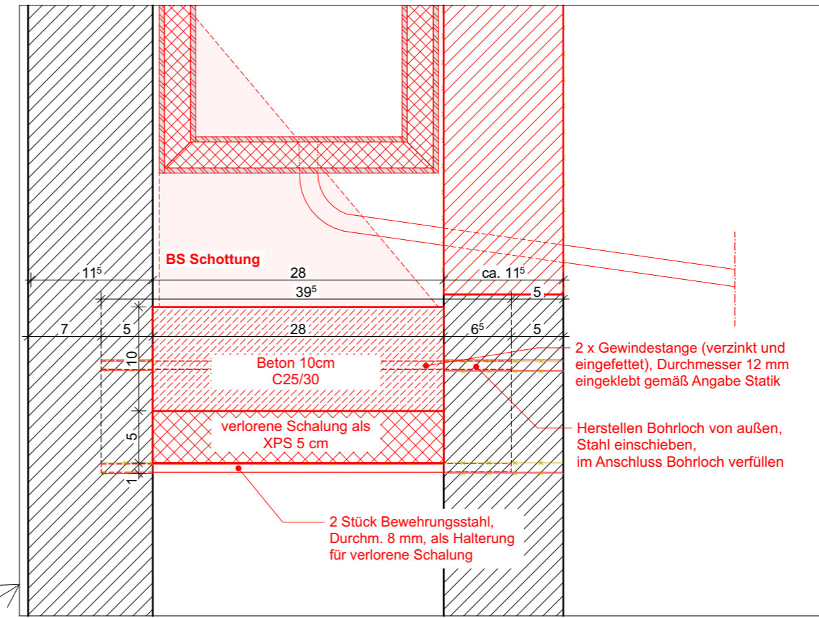
Detail 1 M 1:5
